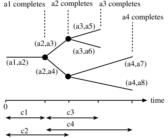
Figure 5: An illustration of how search integrates with action simulation. At time 0, two actions a1 and a2 are being simulated. They have the corresponding completion times c1 and c2 (when may themselves be the result of several critical point jumps in the inner-most simulation loop). When a1 completes, two actions, a3 and a4 are considered to replace it. Action a2 is still present in both search paths, and when it completes, it too is replaced by one of two possible alternative actions. Since both branches of the initial tree are now simulating distinct sets of actions, their completion times no longer line up.
