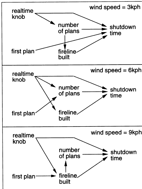
FIGURE 4: The top-ranked models produced by PA for partitions of the Phoenix dataset by wind speed.
