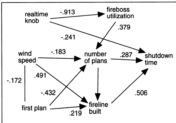
FIGURE 2: A path model derived from Pheonix data.
