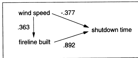
FIGURE 1: A path model of the influences of wind speed and fireline built on shutdown time.
