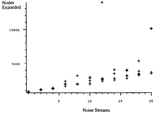
Figure 2: The number of search nodes required to find all of the target planning operators in the block-painting robot domain as a function of the number of noise streams.
